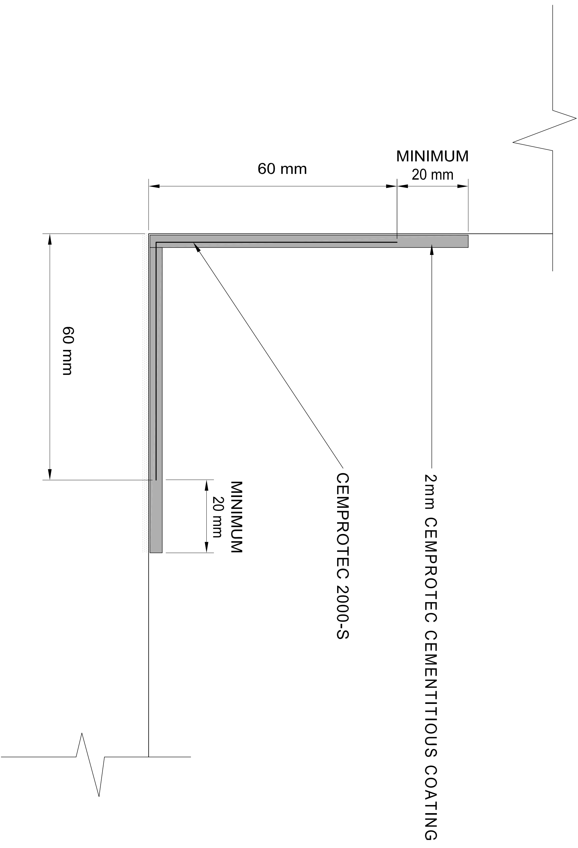
TYPICAL WALL /FLOOR ANGLE
